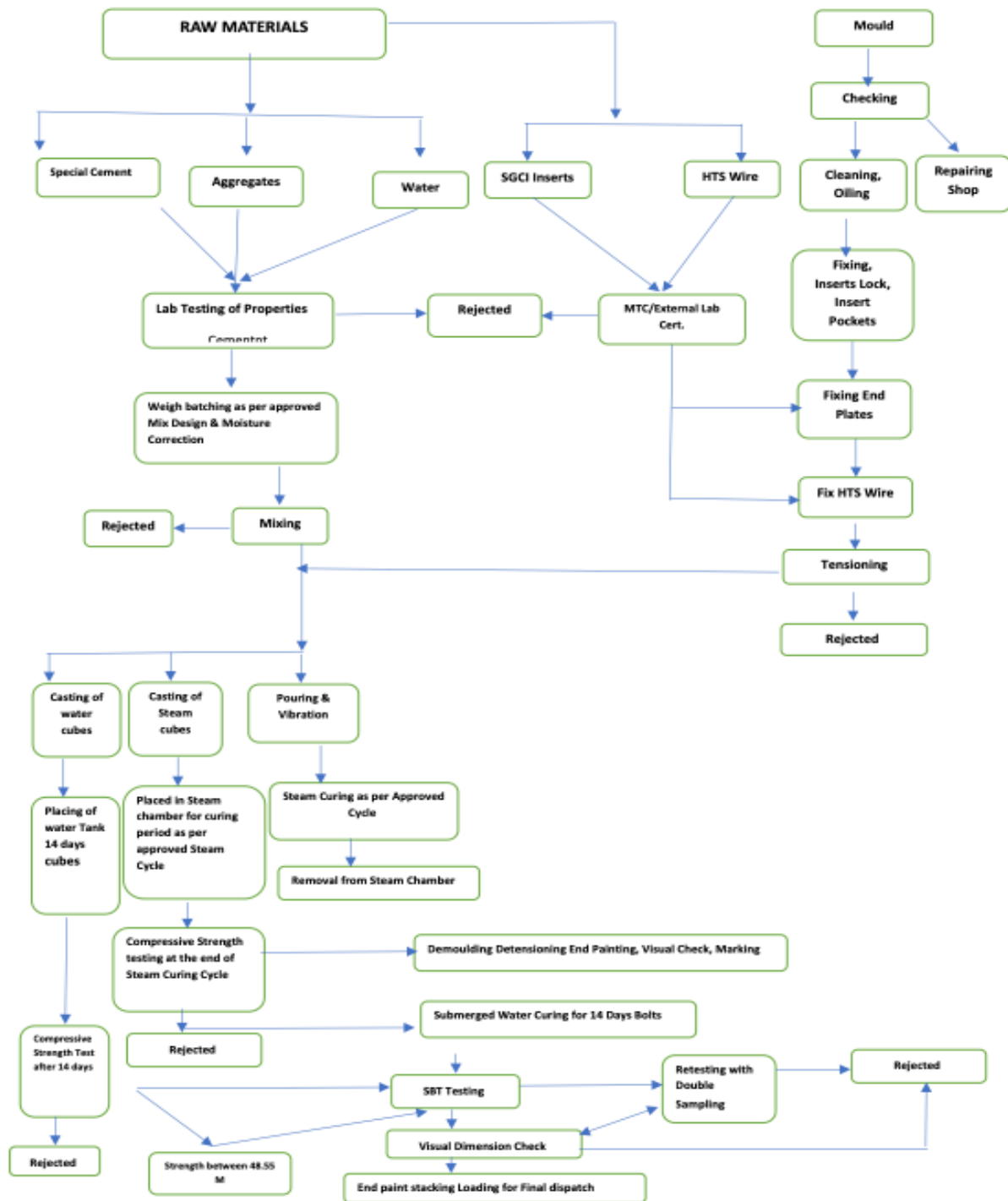
FLOW CHART FOR MANUFACTURING PROCESS OF CONCRETE SLEEPER
